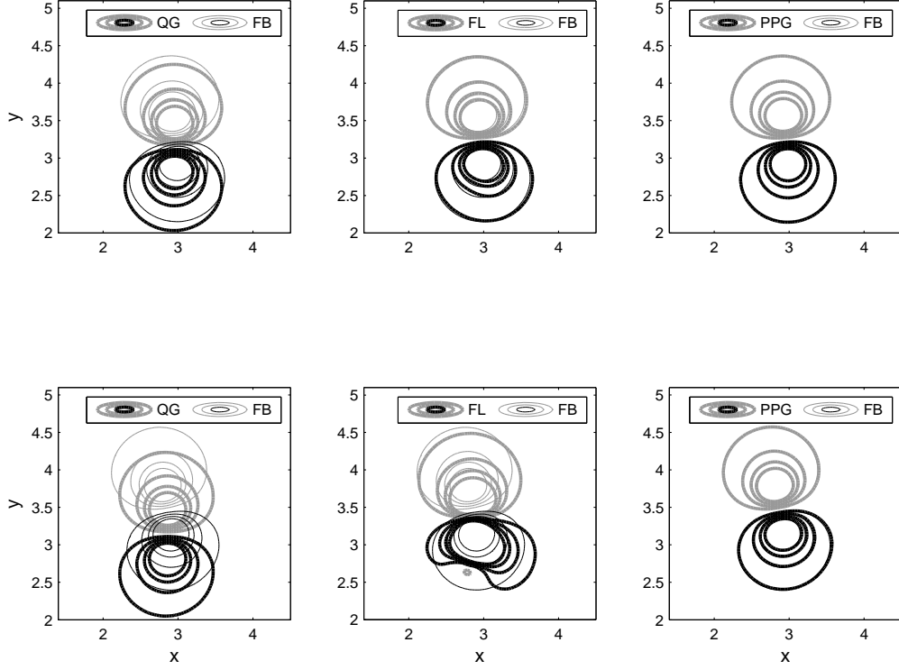
FIGURE 2. Fr = Ro = 0.05 . Contours of the streamfunction with values \psi = \pm 0.25, \pm 0.5, \pm 0.75, \pm 1 at z = \pi and t = 50 (first row); t = 80 (second row). The grey and back lines denote negative and positive values, respectively. In all plots, thin lines correspond to FB contours, while thick lines are the contours corresponding to one of the models: QG (left), FL (middle), PPG (right). The position of the dipoles has been shifted to the center of the domain.
