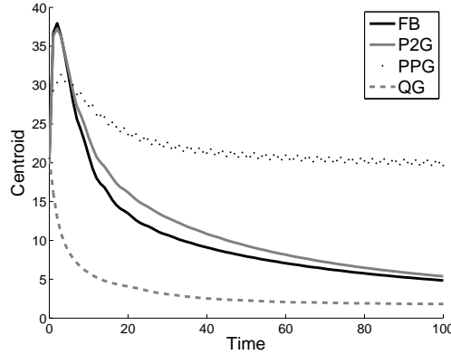
FIGURE 12. Centroid vs. time in rotating stratified turbulence with Fr = Ro \approx 0.2 .
