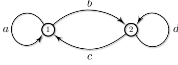
Figure 4: A 2 \times 2 Markov chain.
