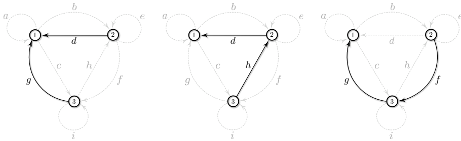
Figure 7: The spanning trees rooted at 1 that define the local spanning tree invariant \tau_1(P) .
