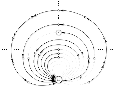
Figure 3: In a loop system at u , the weight of the spanning tree rooted at r \neq u is \rho .
