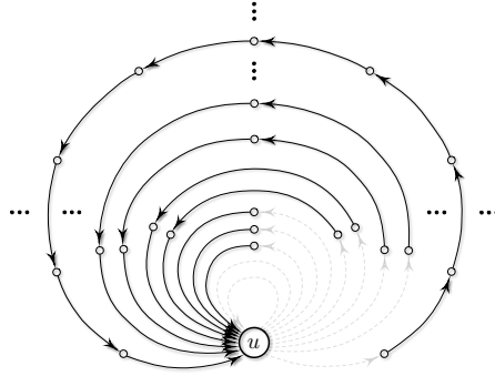
Figure 2: In a loop system at u , the weight of the spanning tree rooted at r = u is 1.
