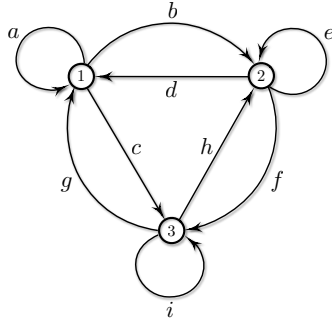
Figure 6: A 3 \times 3 Markov chain.
