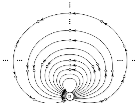
Figure 1: A loop system at u .
