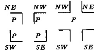
Figure 3: Orthogonal polygons may have these 8 types of vertices.
