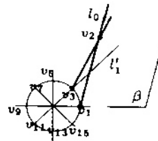
Figure 7: The construction of a polygon that requires floodlights not aligned with its edges.
