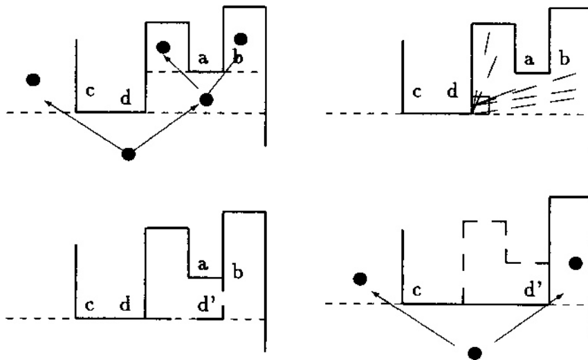
Figure 6: The transformation T that eliminates two reflex vertices, and replaces two leaves and a branch for a region that is a leaf.
