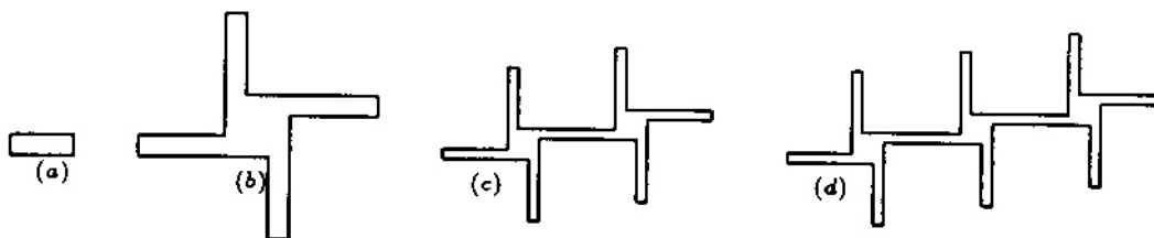
Figure 2: Orthogonal polygons that require one \alpha -floodlight for each tong, when \alpha \in [\pi/2, 3\pi/2) .
