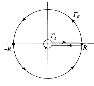
keyhole contour
