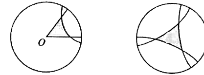
hyperbolic triangles
