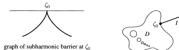
graph of subharmonic barrier at \zeta_0
