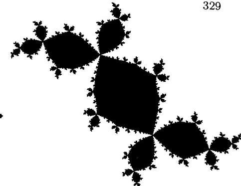
Douady's rabbit ( c = -0.122 + 0.745i )
