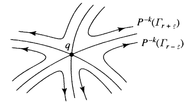
critical point of order m = 2
