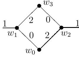
Figure 4.3:
