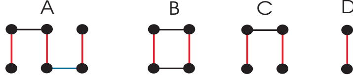
Figure 6.5: Connected components
