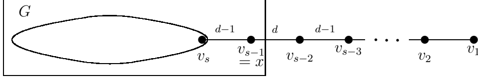
Figure 6.2: Graph \overline{G}_s
