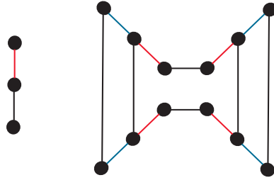
Figure 5.1: Triangle and its extension
