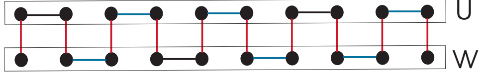
Figure 4.19: The bipartition of the graph P_{4|6}^3
