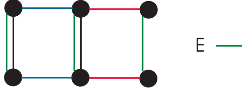
Figure 3.4: Central Involution
