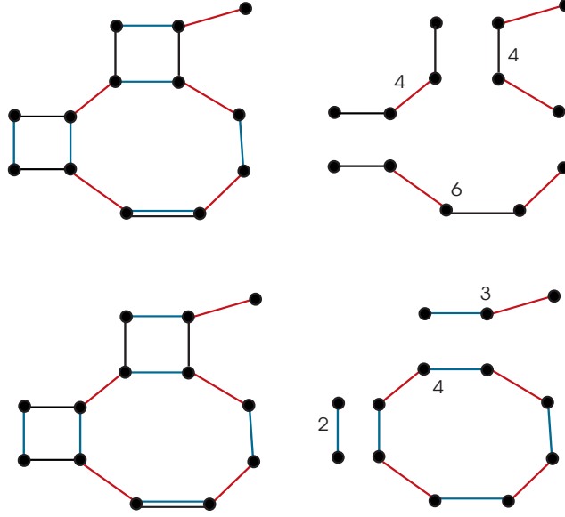
Figure 3.9: \{20, 12\}
