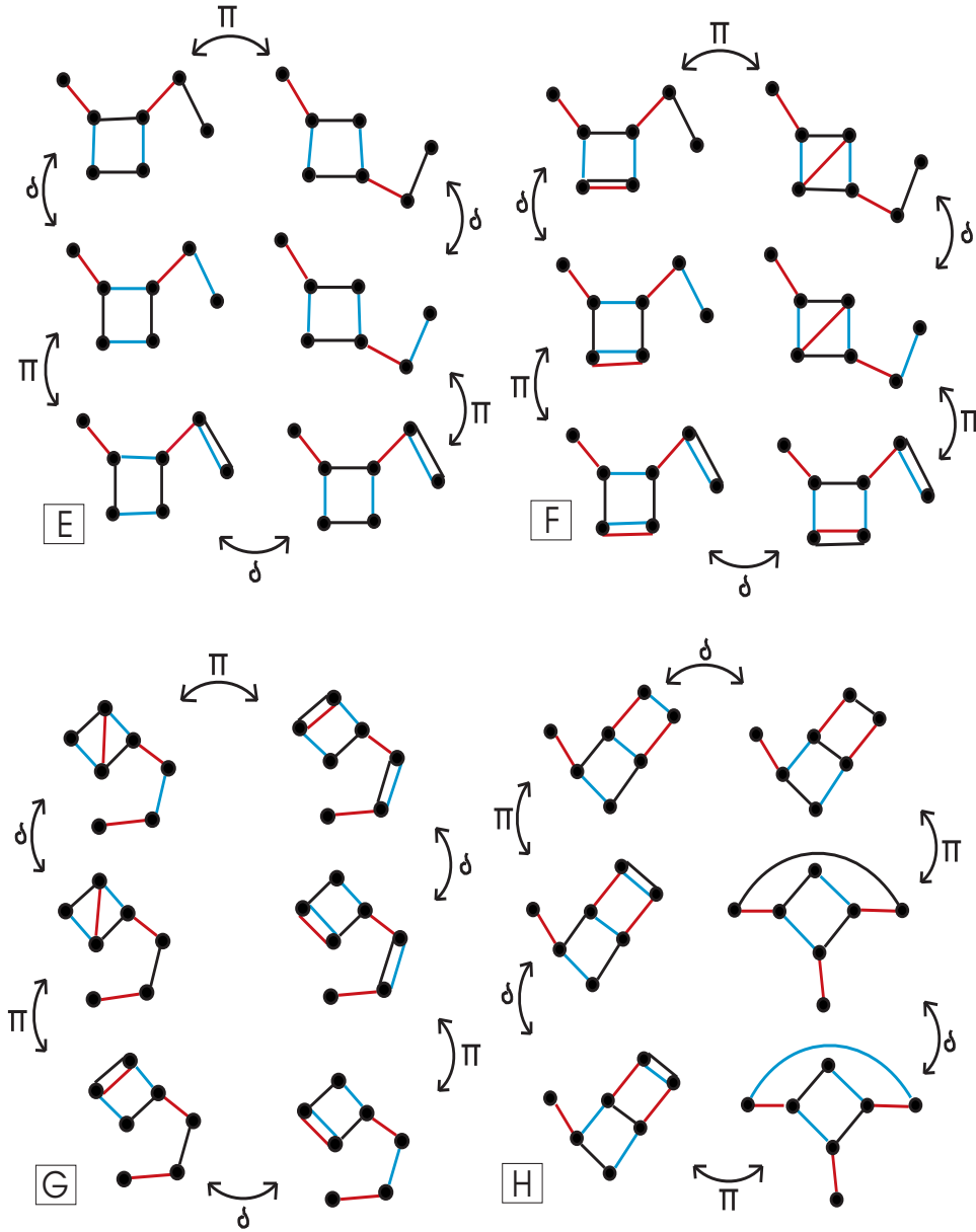
Figure 4.8: Graphs of S_7
