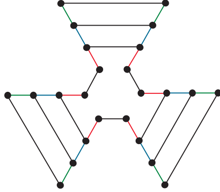
Figure 5.5: CPR graph of 2 \cdot 3^{\{3,3\}-1}
