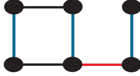
Figure 6.6: Connected components
