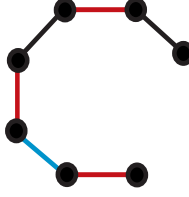
Figure 4.5: \{10, 4\}
