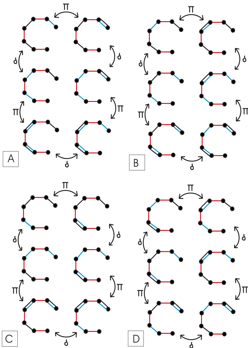
Figure 4.7: Acyclic graphs of S_7
