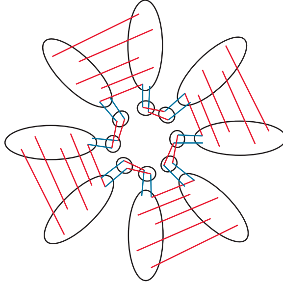
Figure 5.3: G^{2s}
