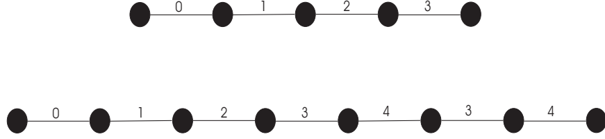
Figure 7.1: The graphs G and G_5 for d = 4
