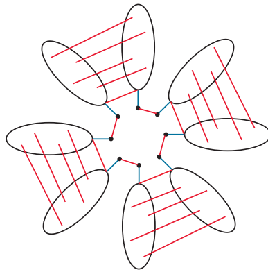
Figure 5.2: G_{2s}
