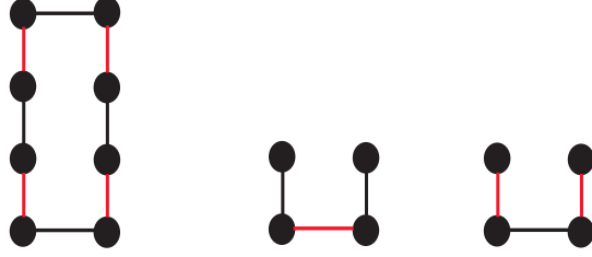
Figure 5.8: Connected CPR graphs of the square
