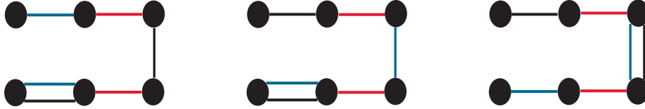
Figure 4.12: CPR graphs of hemidodecahedron, hemiicosahedron and hemigreat dodecahedron
