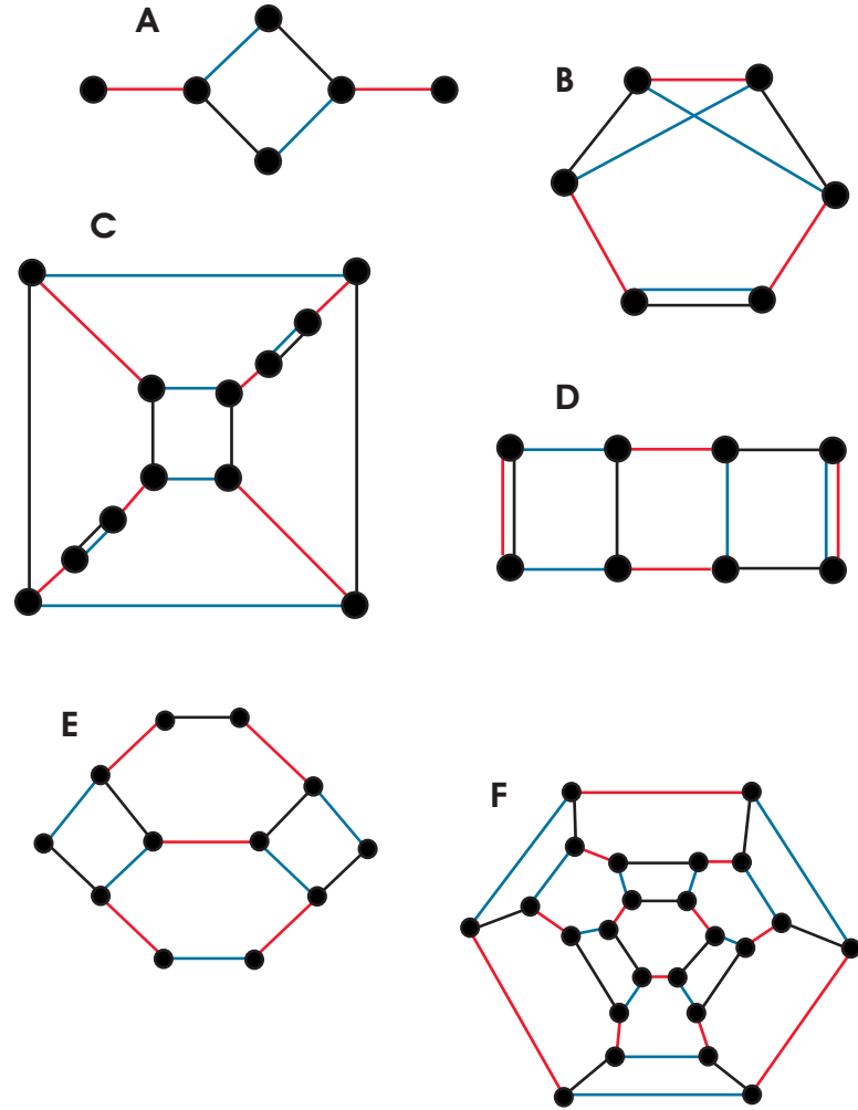
Figure 3.2: Tetrahedron CPR-graphs
