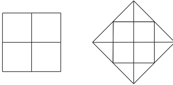
Figure 2.2: The toroids \{4, 4\}_{(2,0)} and \{4, 4\}_{(2,2)}
