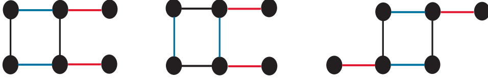
Figure 4.11: CPR graphs of hemicube, hemioctahedron and tetrahedron
