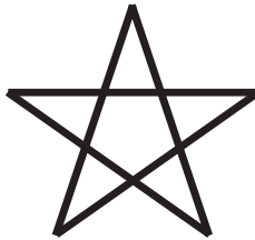
Figure 1.1: Pentagram
