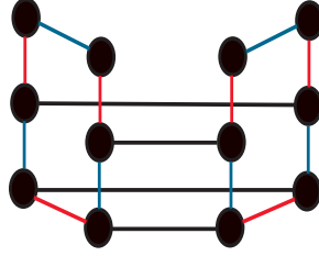
Figure 5.7: CPR graph of the hemicube
