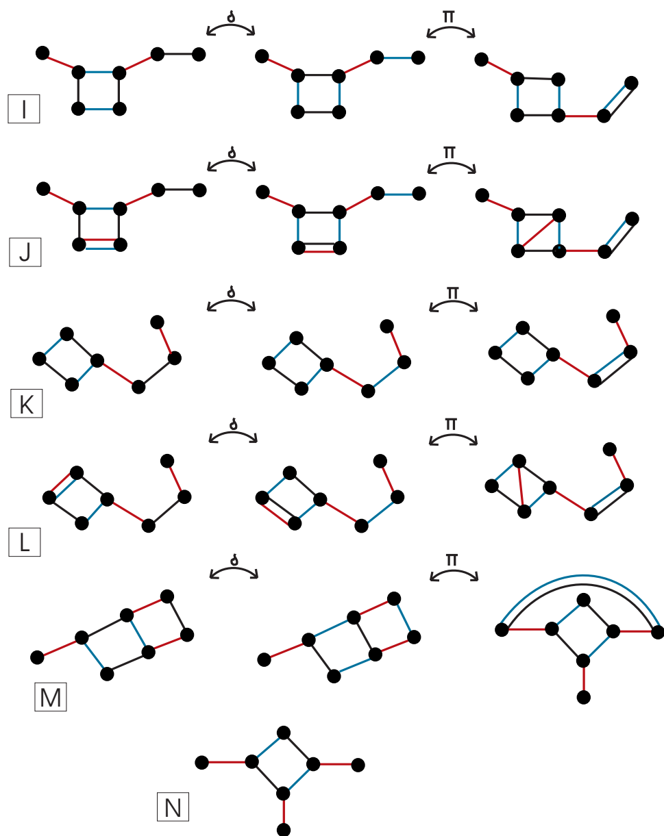
Figure 4.9: Graphs of S_7
