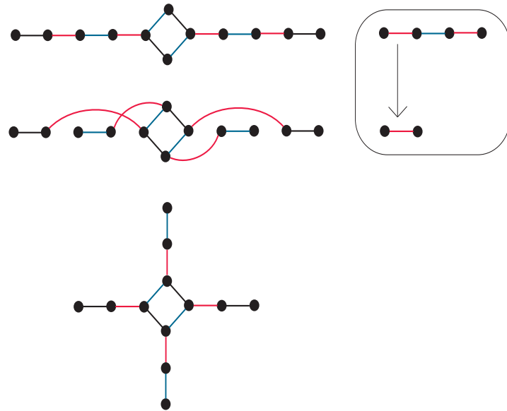
Figure 3.12: Facetting operation
