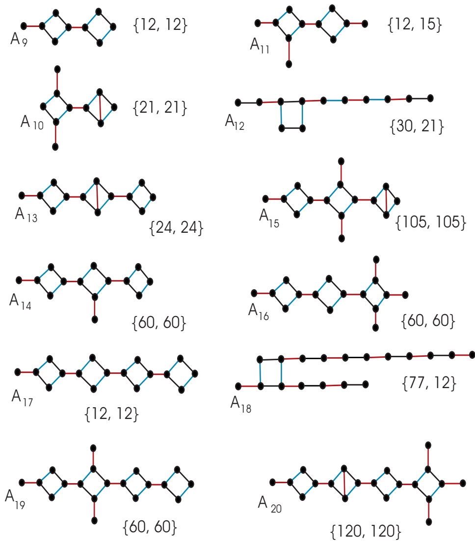
Figure 4.17: Graphs with automorphism group A_n
