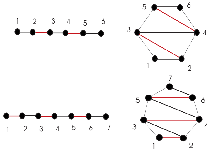
Figure 3.7: D_m acts in the polygon
