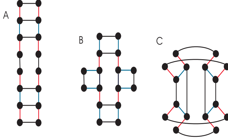
Figure 5.9: CPR graphs of \{4, 4\}_{(4,0)} , \{4, 4\}_{(2,2)} and \{4, 4\}_{(2,0)}
